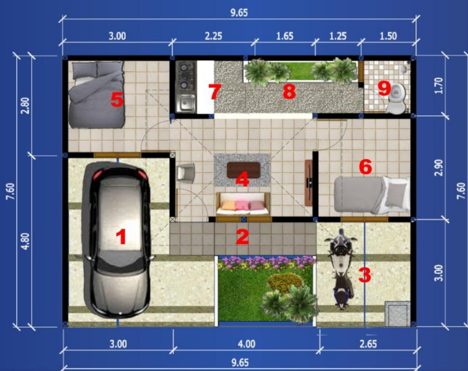
DENAH TYPE 36/73
