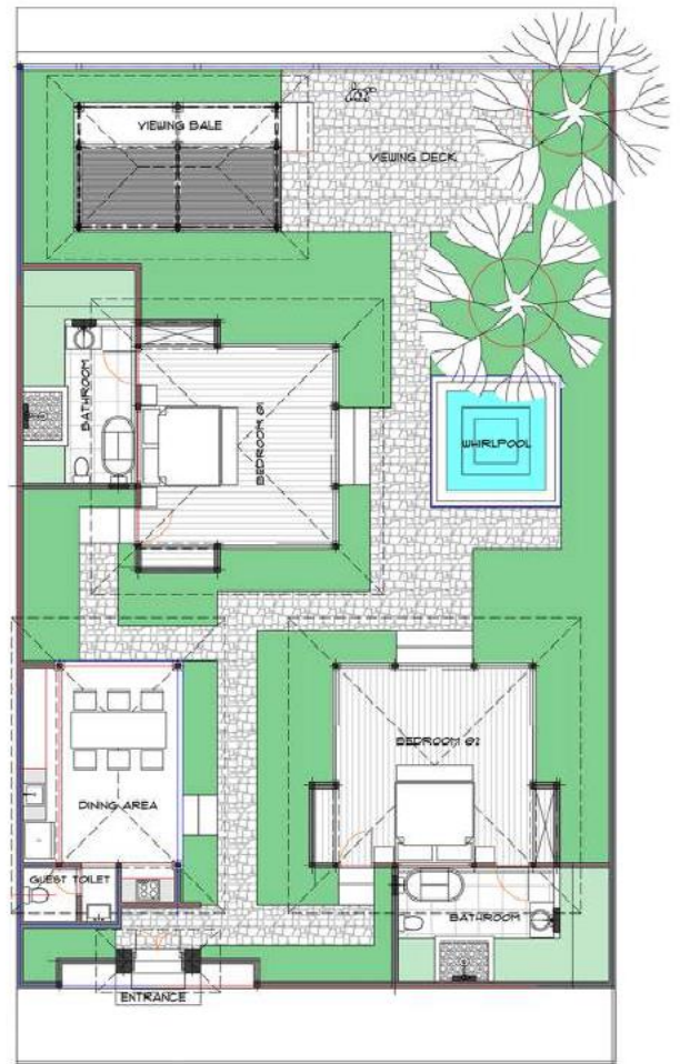
TYPE 2 BR (15 x 24m)
