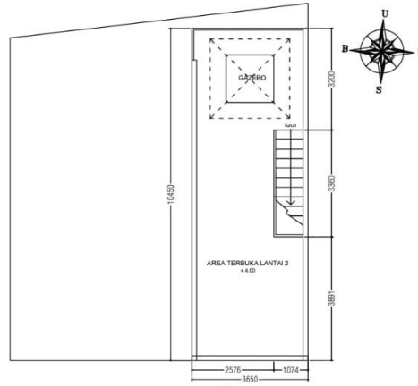
DENAH LANTAI 2 SKALA \frac{1}{4} : 100
