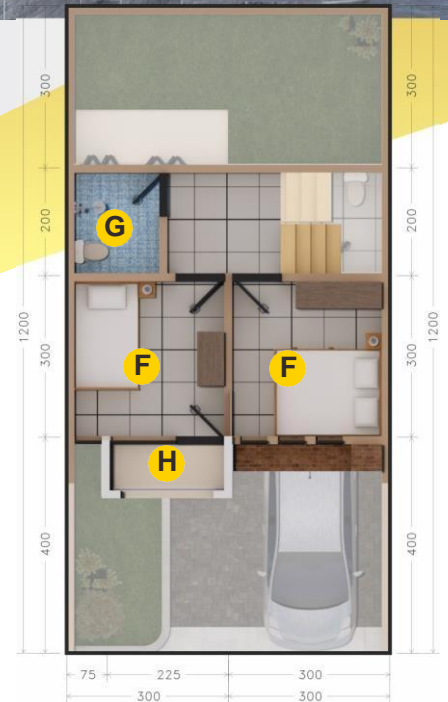
DENAH LT. 2
